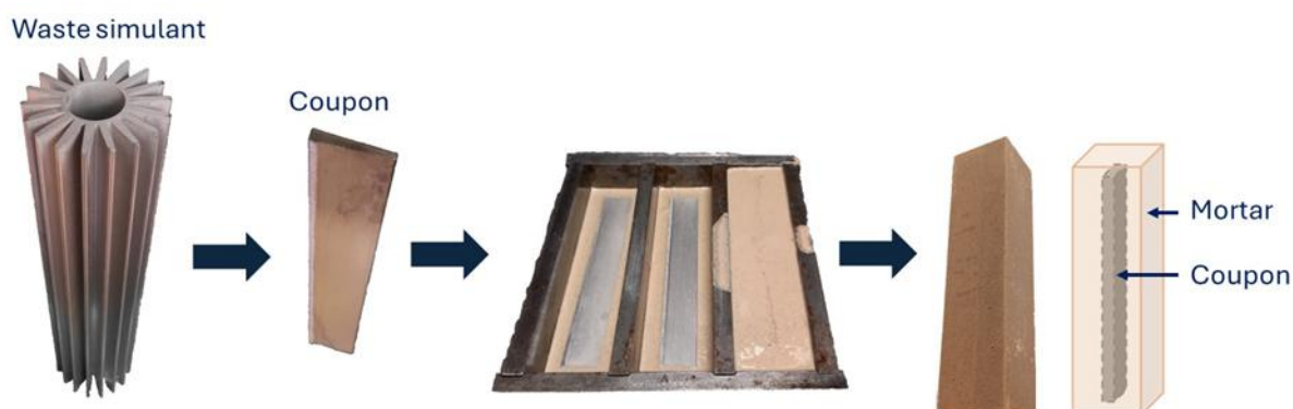
Scheme of immobilization of metallic waste (Mg-Zr alloy used as fuel cladding materials) in MK-geopolymer (courtesy of CEA)
