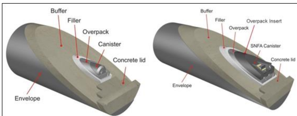
Figure 2-17. Supercontainer components
