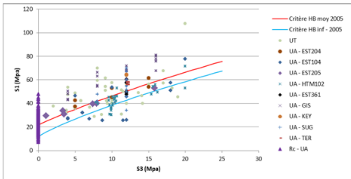
Figure 4-37. Stresses at failure on UT and UA claystone in triaxial tests
