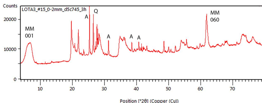
Figure 3-19. XRD data, 0-2 mm sample from the heater (LOT A3, block 15). MM = montmorillonite, A = anhydrite, Q = quartz
