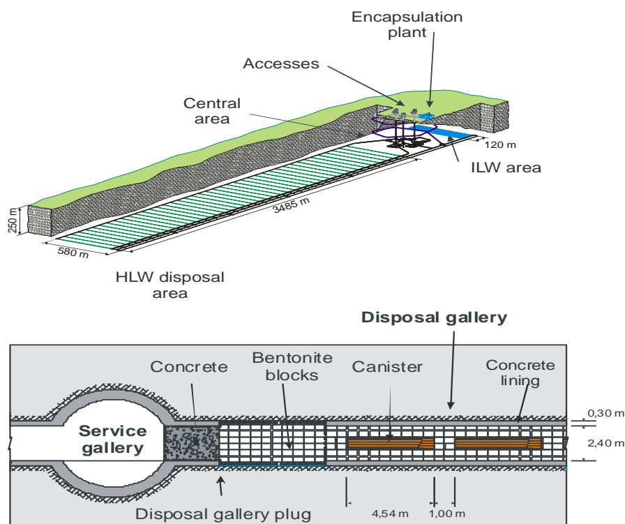
Figure 2-8. Schematic diagram of the geological repository in clay rock (Enresa 2004)
