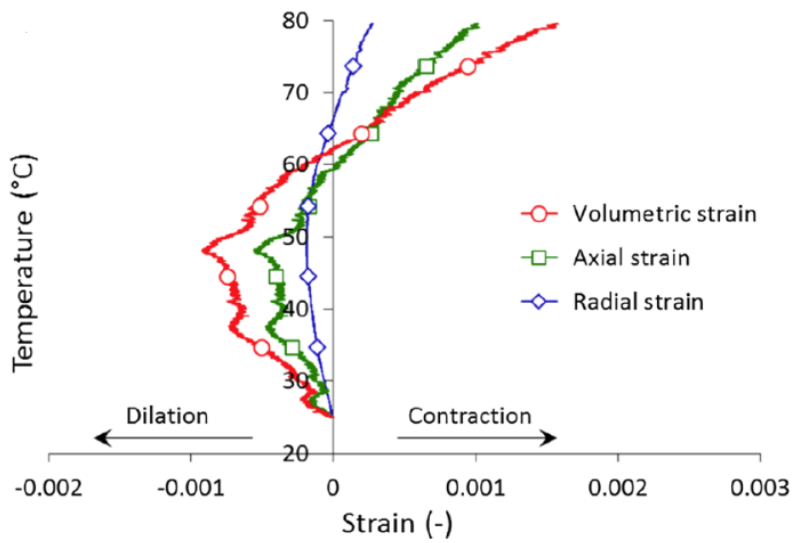
Figure 4-46. Axial, radial and volumetric strain vs. temperature in a drained isotropic compression (Belmokhtar et al. 2017)
