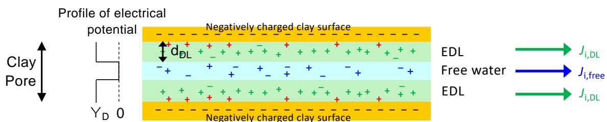
Figure 3-7 – Schematic representation of the Donnan approach for an EDL at the planar clay surfaces. Species in blue (ions in free water) and green colour (ion swarm in the Donnan volume) are assumed to be mobile, while red cationic species are present as immobile surface complexes in the Stern layer. If a concentration difference of a tracer cation species between left and right side of the clay (in analogy to Figure 3-6) is present, the individual flux contributions ( J_i ) would result from the local concentration gradients parallel to the clay surface in the different domains.
