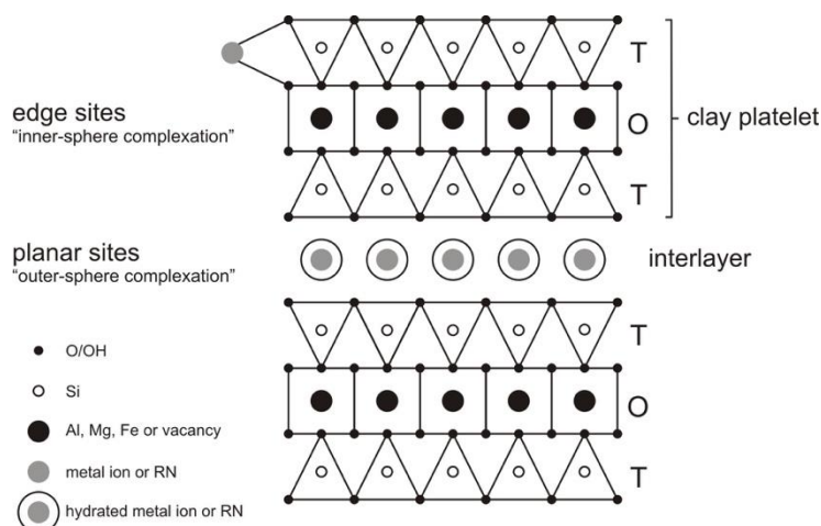
Figure 2-1 – Graphical representation of the structure of 2:1 clay minerals and the different adsorption sites. Taken from Marques Fernandes et al. (2012). Ion-exchange takes place on the permanent charged planar sites in the interlayer and surface complexation takes place at amphoteric sites at the edges.
