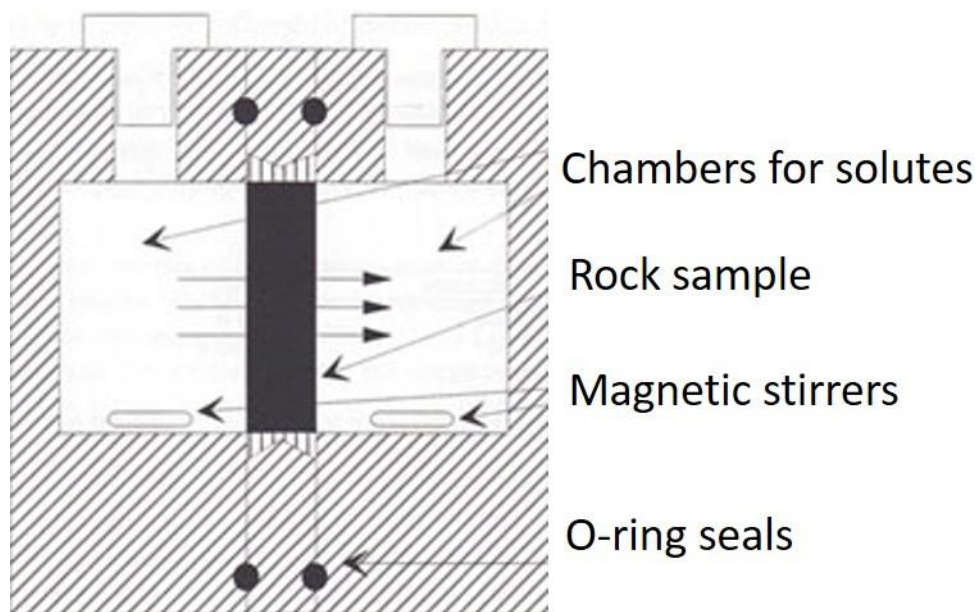
Figure 3-15 – During the through-diffusion experiment diffusion takes place in a sample placed between a tracer-containing solution and a tracer-free solution (Voutilainen et al., 2017).
