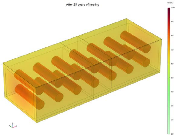
Figure 6-3: Temperatures in Different Panels (a) and in Placement Rooms at Center of Panel 4 (b) after 25 Years of heating from the Coupled THM Integrated Model
