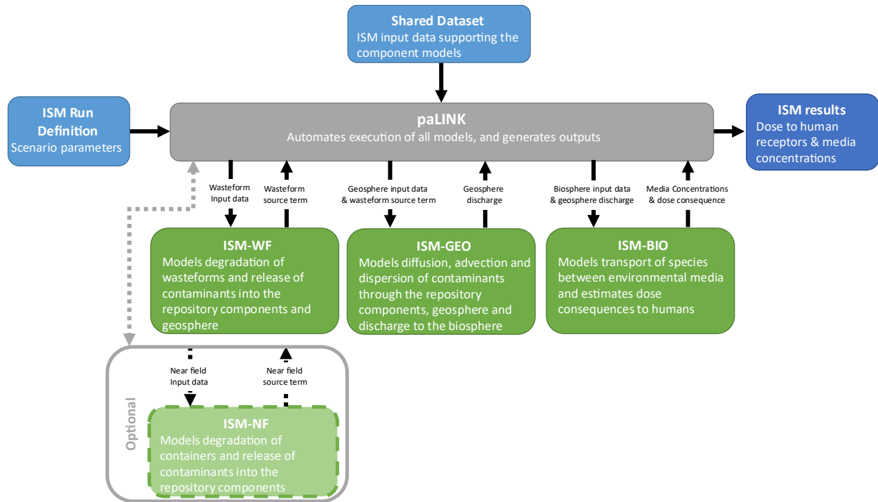
Figure 6-1: paLINK-ISM Configuration
